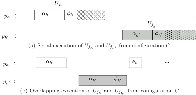
Fig. 3 Illustration for the proof of Lemma 2
